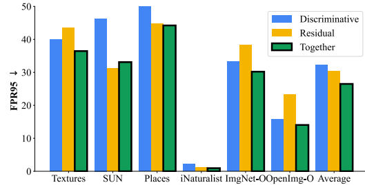
Figure 3: The individual performance in WD and WDR space. Our results demonstrate that two subspaces are effective in detecting OOD data from distinct distributions. Moreover, the integrated score (black border) yields a superior performance compared to each individual, evidencing that our method unifies class-discriminative and class-agnostic information.
