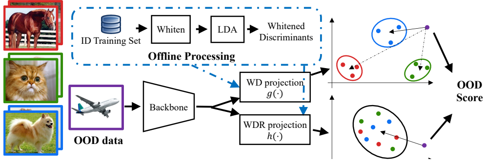
Figure 2: Overview of WDiscOOD method. We detect an OOD sample by projecting the feature into Whitened Discriminative Subspace (WD) and Whitened Discriminative Residual Subspace (WDR) , where ID classes are maximally separated and closely clustered, respectively. The projection functions are obtained from offline Whitened Linear Discriminant Analysis on the ID dataset. OOD samples are presumed to be far from the class clusters in WD space and the entire dataset cluster in WDR space. Therefore, we formulate the OOD score as a combination of the distance to the nearest class centroid in the WD space and to the entire dataset centroid in the WDR space.
