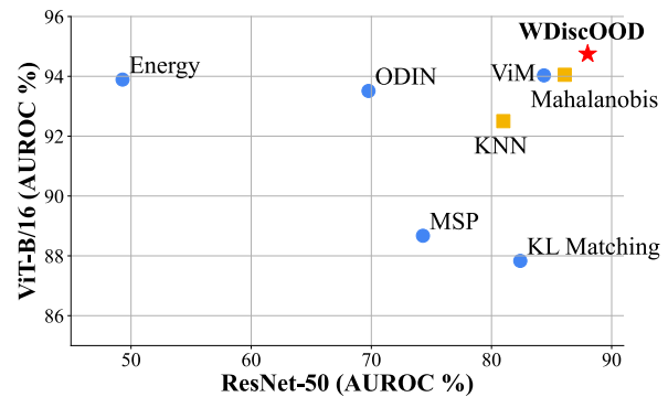
Figure 1: Performance on two OOD detection benchmarks. We propose a novel OOD detection method based on Whitened Linear Discriminant Analysis , which is highlighted with red star. It outperforms baselines with both ResNet-50 (x-axis) and ViT-B/16 (y-axis) model on ImageNet-1k benchmark. Blue dots and yellow square denote classifier-based and feature-based methods, respectively. The AUROCs are averaged over six OOD datasets, for which the detailed results are tabulated in Tab. 1.
