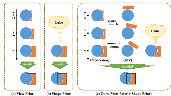
Figure 1: Illustrations of the difference between view prior, shape prior, and our model. While SaVos [35] draws support from the optical flow to realize the view prior, image-level amodal segmentation algorithms typically just utilize the shape prior brought in by the supervision signals. Consequently, they are limited by camera motion and complicated object types, respectively. Unlike the previous methods, beyond the mergence of those two priors, EoRaS utilizes view prior by object-centric learning and further introduces the BEV space where obstruction doesn't exist, which enables our EoRaS to easily handle complex scenarios.
