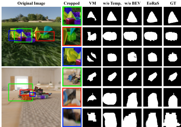
Figure 6: Visualizations derived from models with/without proposed temporal or BEV module. Clearly, the complete model deduces the best full mask, and both the temporal and BEV module can bring consistent benefits.
