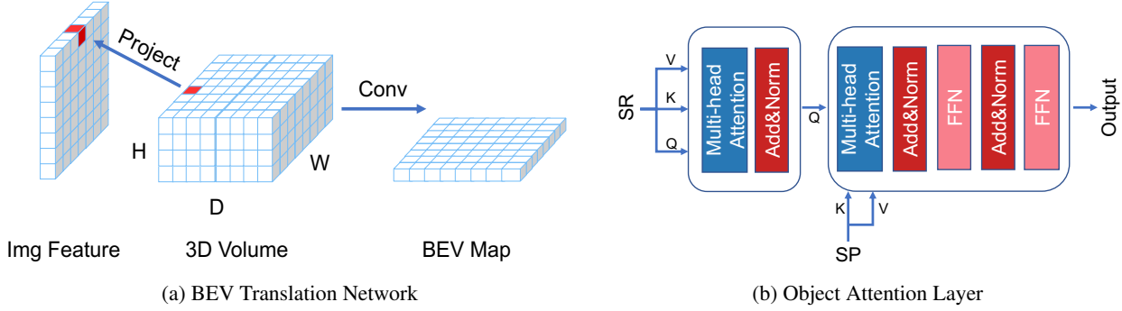
Figure 3: (a) A three-dimensional cuboid is built and rasterized in the camera coordinate. For each voxel, we use the intrinsic matrix to obtain its coordinates in the plane system, and use bilinear interpolation on the front-view features to obtain its feature. Then, a convolutional network is used to obtain the bev map. (b) Our object attention layer in the multi-view fusion layer is stacked by self-attention, cross-attention, and feedforward network. This layer is designed for shape information fusion and takes two variables as input. We nominate the variable to be updated as shape receiver (SR) and another one as shape provider (SP).
