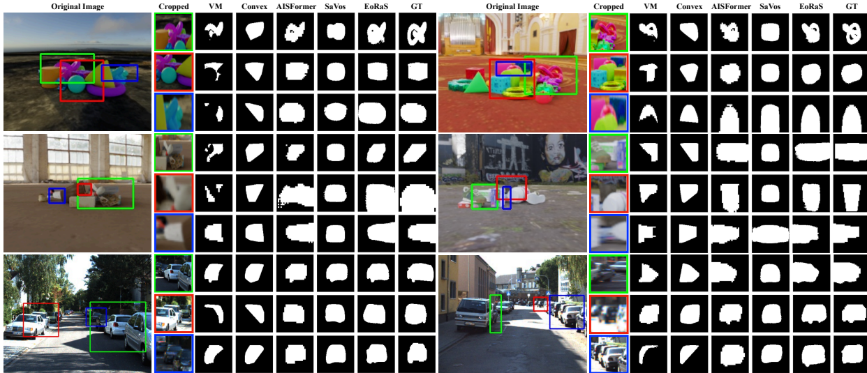
Figure 5: Qualitative comparison between our EoRaS and competitors. From top to down, the three rows are from Movi-B, Movi-D, and KITTI, respectively.
