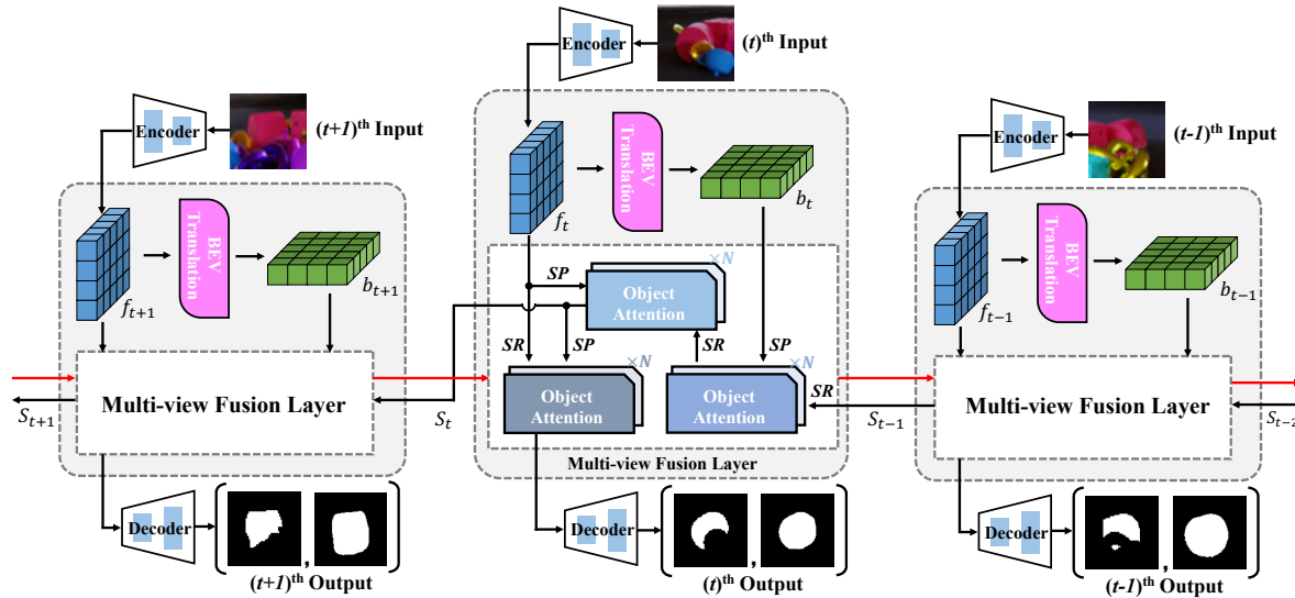
Figure 2: A schematic illustration of our method. The novelty of this architecture mainly lies in the BEV translation network and the multi-view fusion layer. The SP and SR represent the shape provider and receiver (see Section 3.1 for detail), respectively.
