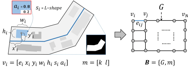
Figure 3: Graph Representation. Our method represents any city block B using a normalized stubby graph representation G (i.e., a grid graph with many columns and few rows), and a set of graph-level features m . Canonical spatial transformation finds the main axis (blue line) of an arbitrary city block, and transforms each node’s spatial information by the relative distance to the main axis.
