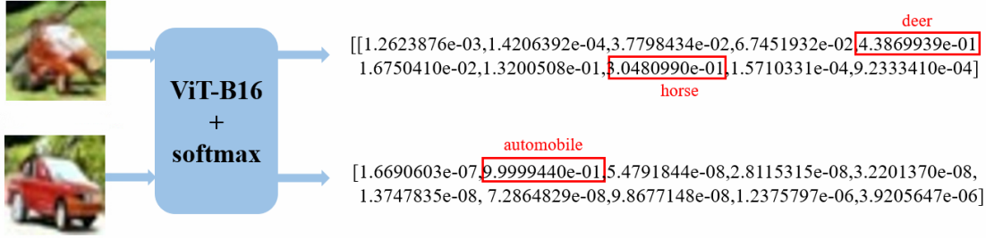
Figure 5. Examples of verifying mode mixture indicator. The image of the top row and the bottom row are judged as existence and nonexistence mode mixture by the indicator in Eq. (17).
