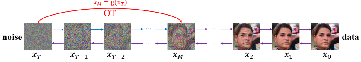
Figure 1. The framework of the proposed DPM-OT . The red curve indicates the Optimal Trajectory , which is induced by the SDOT map g(\cdot) between \mathbf{x}_T and \mathbf{x}_M . Correspondingly, the blue line indicates the first T-M steps inverse diffusion of the vanilla DPM.
