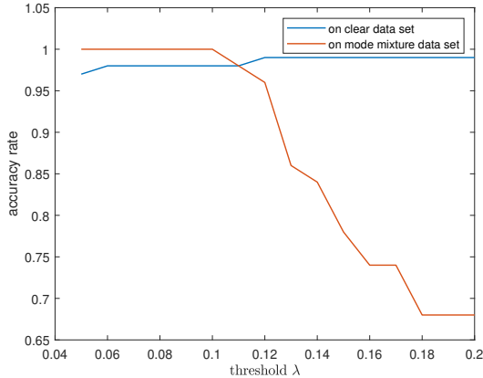
Figure 6. Randomly chosen mixed and unambiguous images to obtain the mode mixture indicator results under different thresholds.
