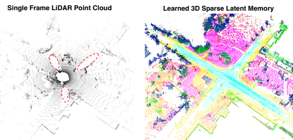
Figure 1. Objects could be partially occluded in single frame LiDAR point cloud. Our approach learns a 3D latent memory representation for better contextualizing the online observations. We apply PCA [14] to reduce the latent dimension to 3 and plot as RGB. (Best viewed in color and zoomed-in.)
