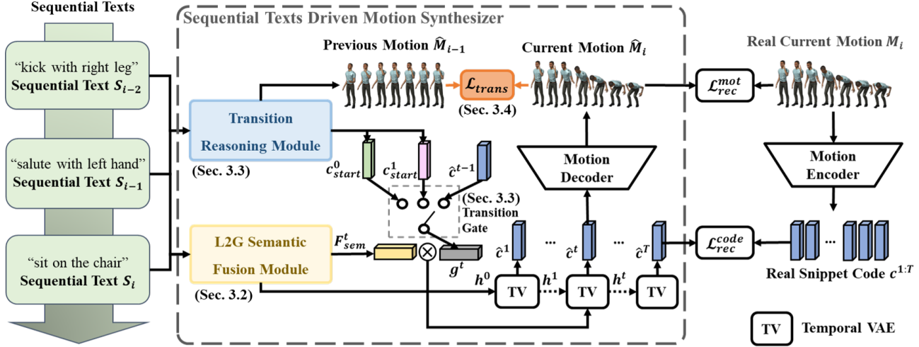
Figure 3: Method Overview: Our model takes sequential texts as input. In the local-to-global (L2G) semantic fusion module, the previous text’s global features and the current text’s local features are fused and extracted. In the transition reasoning module, the motion snippet code at the transition of adjacent motion ( c_{start}^0 and c_{start}^1 ) is deduced from the previous motion. Input the gate snippet code g^t and the semantic text feature F_{sem}^t to synthesize the motion snippet code \hat{c}_i^t . The transition loss further limits the fluency of the transition with the previous motion.
