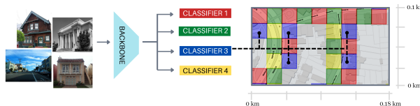
Figure 2. Architecture of Divide&Classify. The different groups, and their relative classifiers, are color coded. The picture explicates how cells are distributed into groups.
