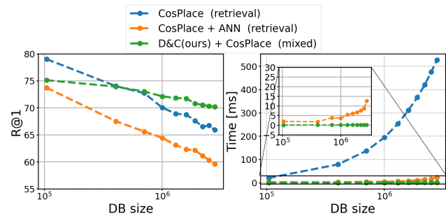
Figure 1. Experiments demonstrating the scalability problem of retrieval-based VPR methods, using the state-of-the-art CosPlace (with exhaustive kNN and with Approximate Nearest Neighbor - ANN - search through Inverted File Index with Product Quantization, IVFPQ). Combining our Divide&Classify method with the retrieval approach yields an optimal performance-efficiency trade-off when scaling up to the city-wide setting.
