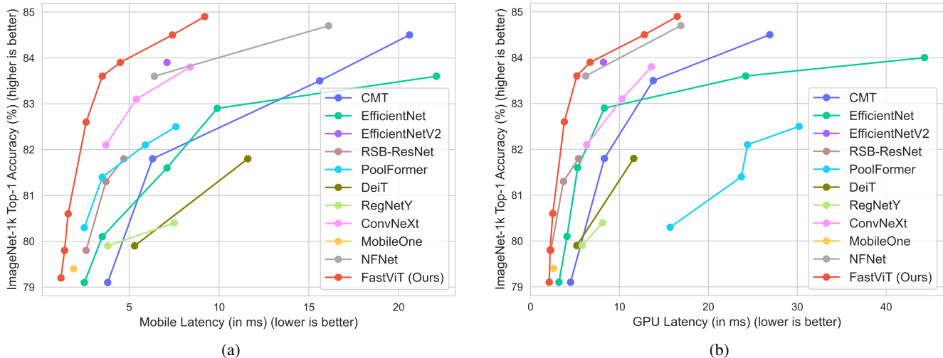
Figure 1: (a) Accuracy vs. Mobile latency scaling curves of recent methods. The models are benchmarked on an iPhone 12 Pro following [55]. (b) Accuracy vs. GPU latency scaling curves of recent methods. For better readability only models with Top-1 accuracy better than 79% are plotted. See supplementary materials for more plots. Across both compute fabrics, our model has the best accuracy-latency tradeoff.
