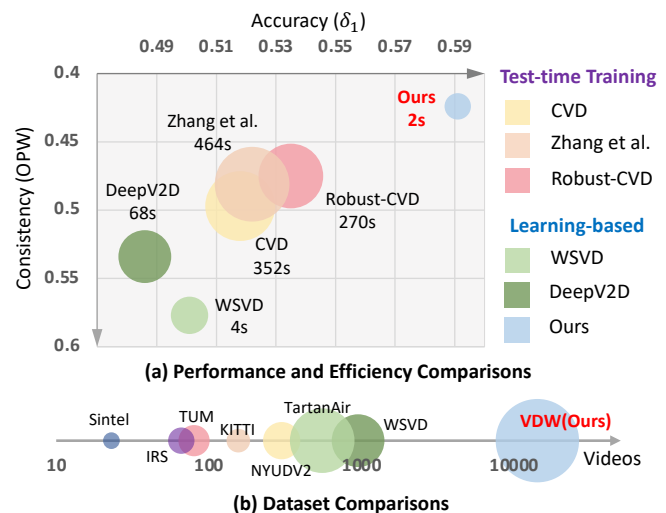
Figure 1: (a) Performance and efficiency comparisons. Circle area represents inference time. Smaller circles mean faster speed. The X-axis represents \delta_1 on Sintel [4] dataset for spatial accuracy. The Y-axis represents consistent metric OPW . Lower OPW means better temporal consistency. Our framework outperforms prior arts by large margins. (b) Dataset comparisons. Larger circles mean larger amounts of frames. We present VDW dataset, the largest video depth dataset in the wild with diverse scenes.
