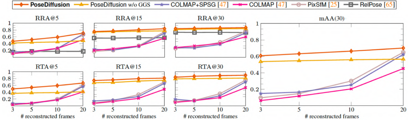
Figure 5: Pose estimation accuracy on CO3Dv2. Metrics RRA@_\tau , RTA@_\tau at different thresholds \tau and mAA(30) ( y -axes, higher-better) as a function of the number of input frames ( x -axes). RelPose does not predict camera translation and hence is omitted in the respective figures.
