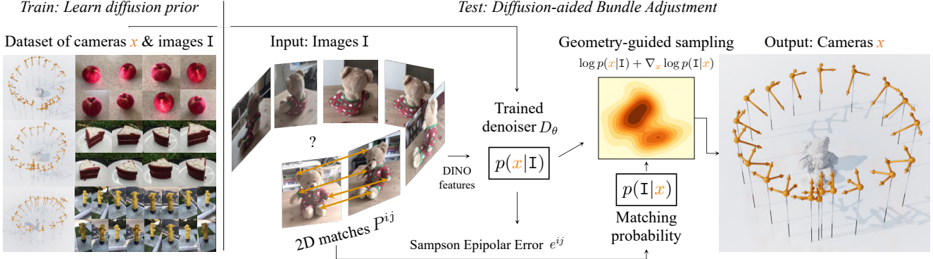
Figure 2: PoseDiffusion overview. Training is supervised given a multi-view dataset of images and camera poses to learn a diffusion model D_{\theta} to model p(x|I) . During inference the reverse diffusion process is guided through the gradient that minimizes the Sampson Epipolar Error between image pairs, optimizing geometric consistency between poses.
