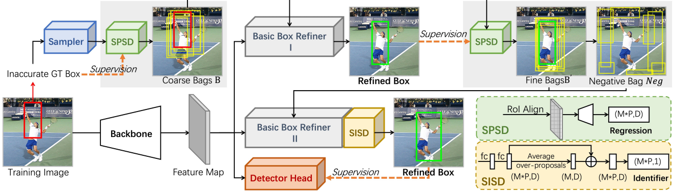
Figure 3: The framework of SSD-Det. It contains basic box refiner, SPSD module, SPSD module and a detector head. Neighborhood sampler is adopted around the inaccurate annotation. Then, SPSD module generates better proposal bags which are fed into basic box refiner for MIL training. The selected proposals are average weighted as the refined box and supervise the next SPSD training. Meanwhile, the SPSD module predicts the IoU between proposals and the object, and the estimated IoU is multiplied by classification score for better proposal selection to generate the refined box. SPSD shares backbone with the detector.
