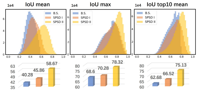
Figure 5: Bag quality (IoU of proposals with GT) of construction in SSD-Det. B.S. (blue) means neighborhood sampler. SPSD I (orange) denotes single SPSD adopted. SPSD II (yellow) is two SPSD and interactive structure adopted. SPSD II significantly improves the quality.
