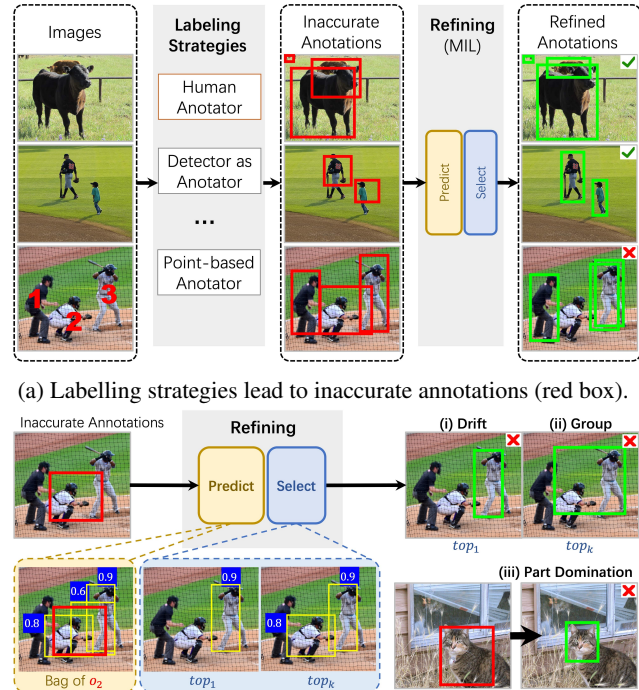
(a) Labelling strategies lead to inaccurate annotations (red box). (b) Three problems during previous MIL refining. Because their selections depend solely on classification, (i,ii): the refined box (green box) drifts to another object or makes a group prediction (merging across multiple objects) due to neighbor disturbance. Yellow boxes are proposals in the middle person's MIL bag. (iii): Local part may be more discriminative than the entire object and will be predicted.
