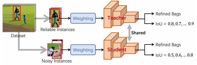
Figure 2: The mechanism of Spatial Self-Distillation. By assigning higher weight, the low-noise annotations can be seen as reliable samples to guide the training of proposals’ spatial position and identity learning in SPSD and SISD.
