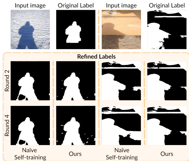
Figure 2. Comparison of label quality produced by a naive self-training framework and our SILT framework. Our SILT framework generates more accurate labels with finer details.
