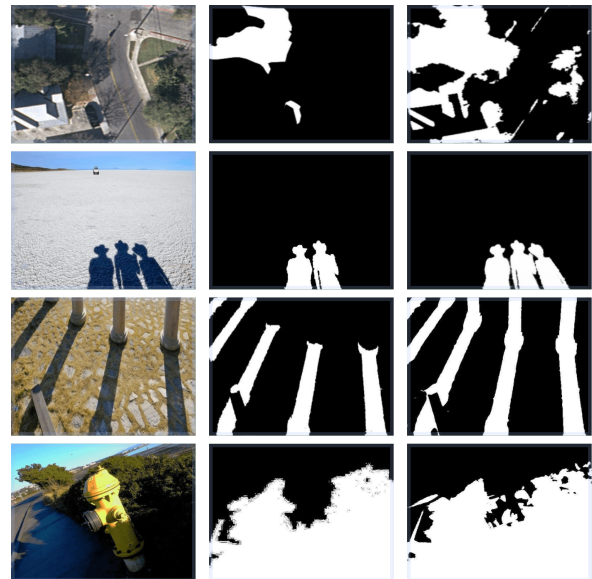
(a) Training images in existing datasets (b) Original labels in existing datasets (c) Our refined labels
