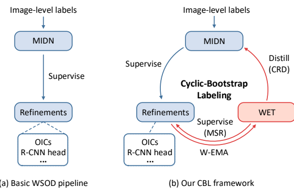
Figure 1. Comparison between the basic WSOD pipeline and our proposed CBL framework (feature extractor is omitted for simplicity). In the CBL framework, the subsequent refinement modules of MIDN are finally utilized to distill MIDN in turn, forming a cyclic-bootstrap procedure.
