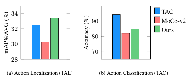
Figure 1. Comparison of Kinetics-400 pre-trained models by fine-tuning on downstream TAL (ActivityNet v1.3) and TAC (UCF101) datasets. ‘TAC’ means supervised TAC pre-training, and we treat MoCo-v2 [16] with video input as our baseline. Instance-level discrimination is not well-aligned with TAL, thus unsupervised pre-training tailored for TAL is on demand.
