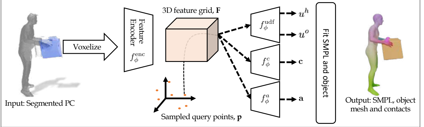
Figure 1: The BEHAVE network takes voxelized human and object point cloud as input and generates an input aligned 3D feature grid, F . We then sample 3D query points and for each input point p , we use the point feature F(p) to predict unsigned distance to human and object surfaces, u^h , u^o , correspondences to the SMPL model c and object orientation a . We use these predictions to fit SMPL and object meshes to the input, explicitly taking the contacts between them into account.
