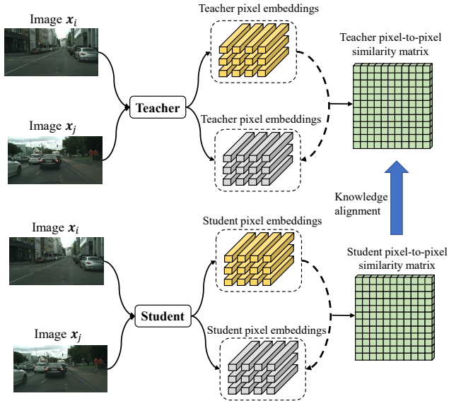
Figure 1. Overview of mini-batch based pixel-to-pixel distillation.
