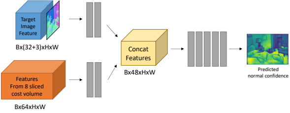
Figure 2: The inputs are processed with two mini-branches (with 2 layers of 3x3 convolutions), and then jointly fed into 5 dilated convolutions followed by final sigmoid activation to regress the normal confidence map.
