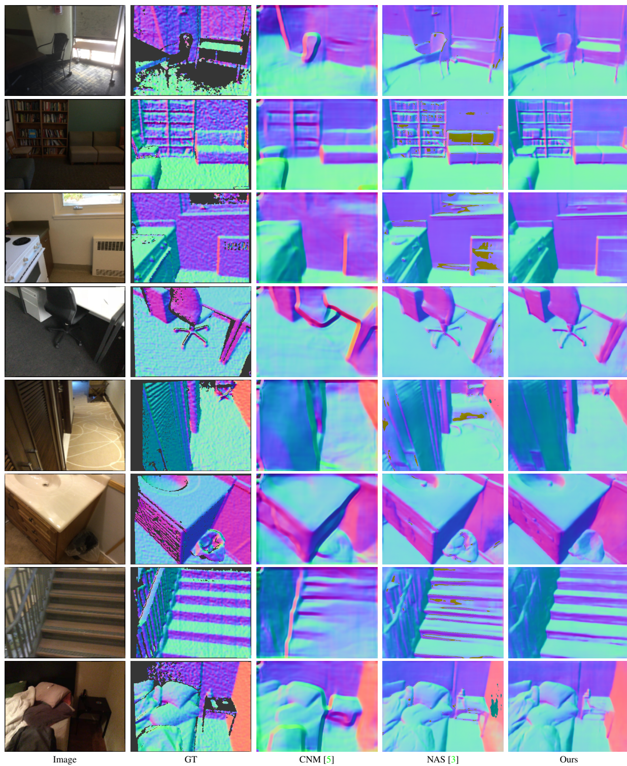
Figure 4: More qualitative results of surface normal estimation on ScanNet [1]. Better viewed when zoomed in.
