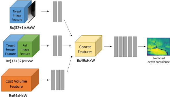
Figure 1: The inputs are processed with three mini-branches (with 2 or 3 layers of 3x3 convolutions), and then jointly fed into 5 dilated convolutions followed by final sigmoid activation to regress the depth confidence map.
