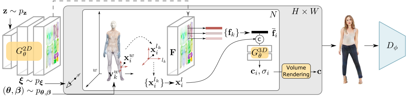
Figure 2: Generative VeRi3D. We model the generative human radiance fields based on a set of vertices and their corresponding feature vectors. Given a sampled camera pose \xi and sampled human pose and shape (\theta, \beta) , we sample a 3D point \mathbf{x}_i^w along a ray in the observation space and retrieve its K nearest neighbors \{\mathbf{v}_k^w\}_{k=1, \dots, K} . For each neighboring vertex \mathbf{v}_k^w , we transform \mathbf{x}_i^w to the local coordinate system of \mathbf{v}_k^w and obtain \mathbf{x}_i^{l_k} . Next, we combine the weighted feature vectors \{\mathbf{f}_k\} and the local coordinate \{\mathbf{x}_i^{l_k}\} to generate the color \mathbf{c} and density \sigma at this point. This mapping is performed on N sample points on each ray and H \times W pixels to obtain an output image, whereas the feature vectors are generated once using a 2D convolutional network.
