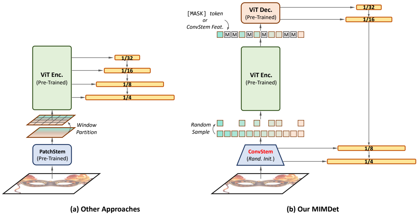
Figure 1: Overview of our MIMDET and comparisons with previous representative approaches adapting vanilla ViT for object detection (e.g., [31]). In MIMDET, a randomly initialized compact convolutional stem (ConvStem) replaces the pre-trained large kernel patchify stem (PatchStem), and the ViT encoder only receives and processes sampled partial input embeddings. The intermediate features of ConvStem can directly serve as the higher resolution inputs for a standard FPN [32].
