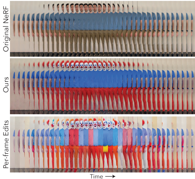
Figure 6: Consistency: Vertical slices of a rendered novel camera path show the consistency across varying viewpoints. The original NeRF rendering (top) is quite consistent, similar to our edited result (middle), using the prompt “turn him into a clown”. Conversely, running InstructPix2Pix [2] on each rendered frame independently results in notable inconsistency, such as varying hair and shirt colors.
