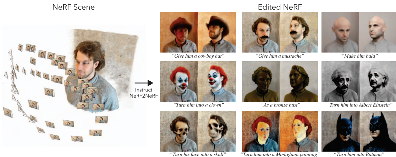
Figure 1: Editing 3D scenes with Instructions. We propose Instruct-NeRF2NeRF, a method for consistent 3D editing of a NeRF scene using text-based instructions. Our method can accomplish a diverse collection of local and global scene edits.
