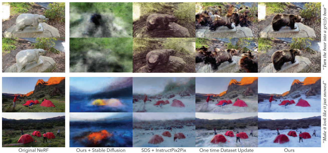
Figure 8: Baseline Comparisons: We compare our model with a collection of variants described in Section 4.1.
