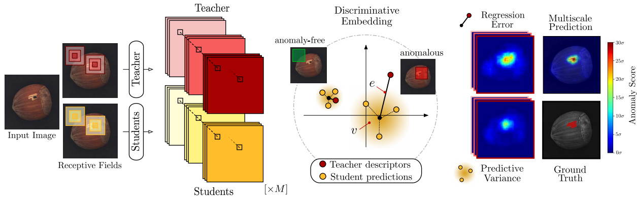
Figure 2: Schematic overview of our approach. Input images are fed through a teacher network that densely extracts features for local image regions. An ensemble of M student networks is trained to regress the output of the teacher on anomaly-free data. During inference, the students will yield increased regression errors e and predictive uncertainties v in pixels for which the receptive field covers anomalous regions. Anomaly maps generated with different receptive fields can be combined for anomaly segmentation at multiple scales.
