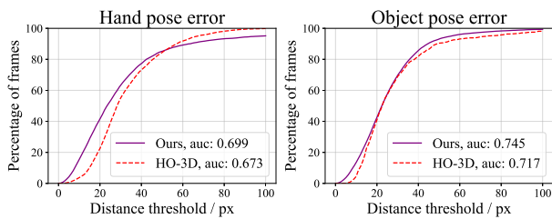
Figure 5. Evaluation of our baseline for hand-object pose estimation on HO-3D. We report the PCK for 2D joint mean-end-point error for hands, and the mean 2D reprojection error for objects.
