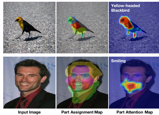
Figure 1. Why does a deep model recognize the bird as “Yellow-headed Blackbird” or consider the person “Smiling”? We present an interpretable deep model for fine-grained recognition. Given an input image (left), our model is able to segment object parts (middle) and identify their contributions (right) for the decision. Results are from our model trained using only image-level labels.
