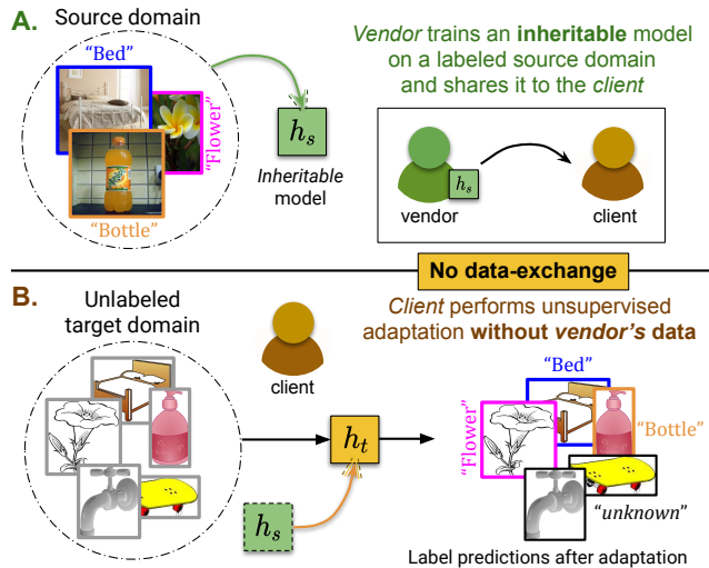
Figure 1. A) We propose inheritable models to transfer the task-specific knowledge from a model vendor to the client for, B) performing unsupervised open-set domain adaptation in the absence of data-exchange between the vendor and the client .
