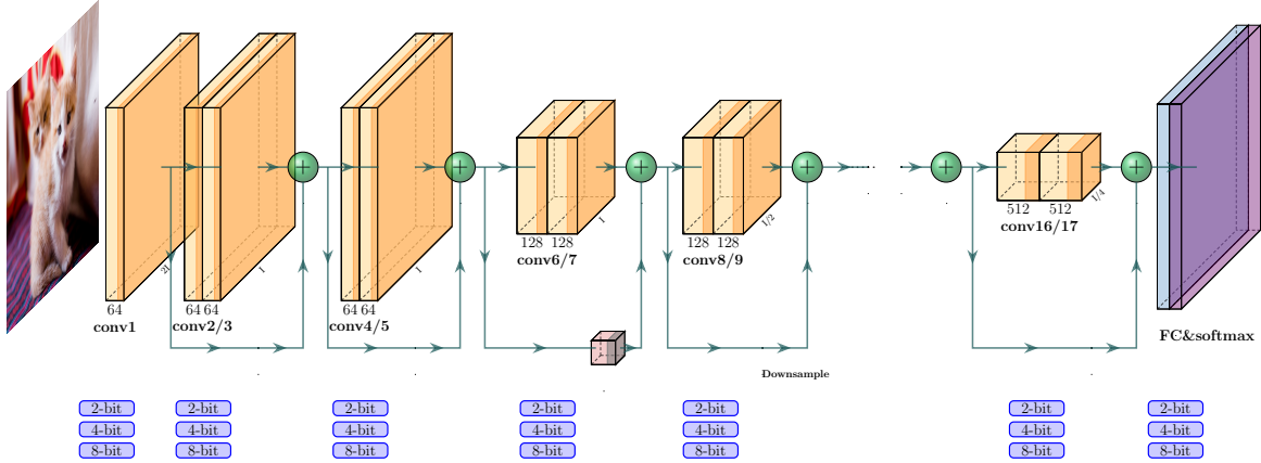
Figure 5: Mixed precision illustration of ResNet18 on ImageNet.
