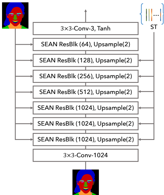
Figure 1: SEAN Generator. The style codes ST and segmentation mask are passed to the generator through the proposed SEAN ResBlks. The number of feature map channels is shown in the parenthesis after each SEAN ResBlk. To better illustrate the architecture, we omit the learnable noise inputs and per-style Conv layers in this figure. These details are shown in Fig.3 of the main paper (see A_{ij} and B_{ij} ).
