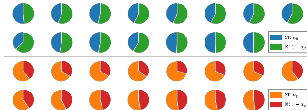
Figure 6: Contributions of ST-branch and Mask-branch for each SEAN normalization block. The pie charts and SEAN normalization blocks are in one-to-one correspondence.
