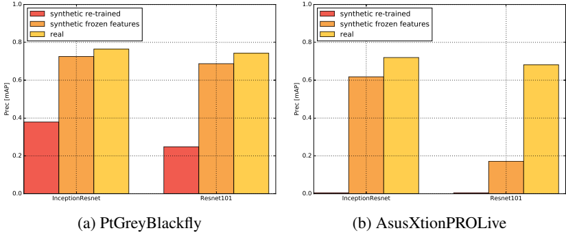
Fig. 5. The effect of freezing the pre-trained feature extractor, for two different cameras. Training the feature extractors on synthetic images performs poorly, and totally fails in the case of the AsusXtionPROLive camera. When using feature extractors pre-trained on real images without retraining them, the performances of detectors trained on synthetic data are almost as good as when training them on real data, except when ResNet101 is used with images from the AsusXtionPROLive camera.
