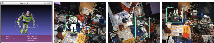
Fig. 1. We show that feature extractor layers from modern object detectors pre-trained on real images can be used on synthetic images to learn to detect objects in real images. The top-left image shows the CAD model we used to learn to detect the object in the three other images.
