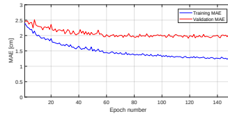
Fig. 4. Mean training (blue) and validation (red) error at each epoch of the K -fold validation.
