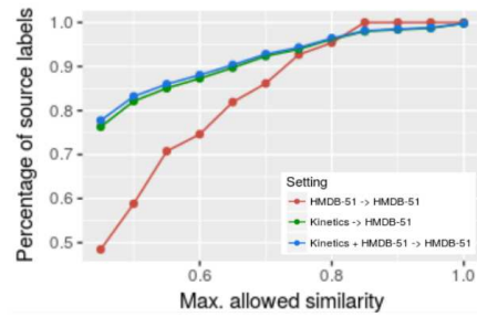
Fig. 3: Proportion of source labels allowed depending on the semantic similarity threshold s_{th} .
