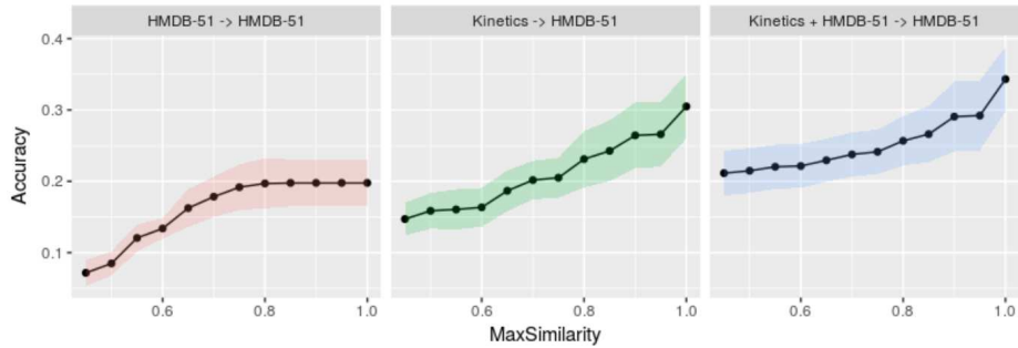
Fig. 4: Influence of source-target label similarity on ZSL performance. X-Axis denotes the semantic similarity threshold s_{th} above which source categories are excluded. Having similar classes in the seen and unseen sets strongly affects accuracy, an effect that is more pronounced when using external datasets.
