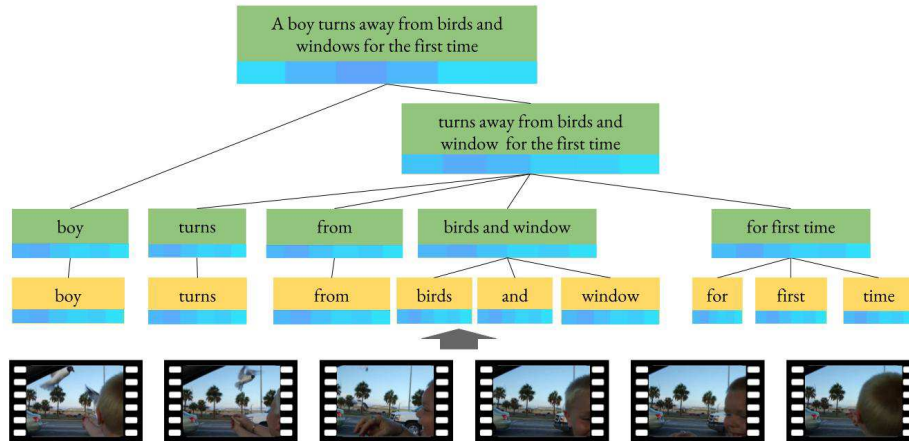
Fig. 3. Qualitative example of TMN evaluated on a query-video pair. Attention maps at base and combine nodes are visualized, where the color bars represent attention weights with darker blue indicating higher weights. Attention maps for the base nodes show the activation of a single word, while the attention map in a combine node shows how information from children are aggregated, and how the modules specifically take in the temporal quality (“for the first time”) of the phrase encoding in each module.
