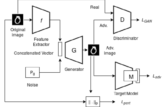
Figure 1: AdvGAN++ architecture.
