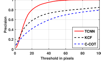
Figure 11: Tracking comparison with precision plot.
