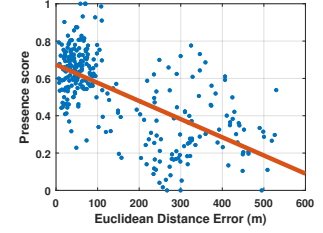
Figure 8: Presence scores vs Euclidean estimation errors.
