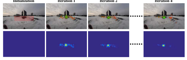
Figure 4: Iterative coupler detection using DCNN. The top row is the input image with the results of (\Delta \mathbf{u}, s) . The green color means s = 1 , and the red is s = 0 . The bottom row shows the results of the weighted sum of Gaussians. Best viewed in color.
