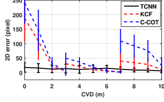
Figure 10: Tracking comparison with errors in pixels.
