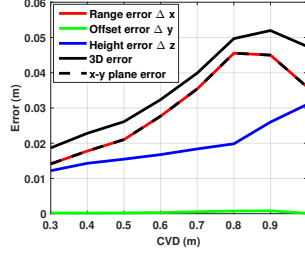
Figure 14: Overall system accuracy on the height label set.
