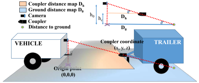
Figure 3: 3D distance estimation of the coupler.
