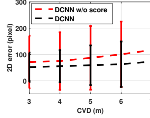
Figure 7: Detection errors vs with distance in meters.
