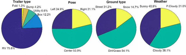
Figure 6: Statistics of the trailer coupler database.
