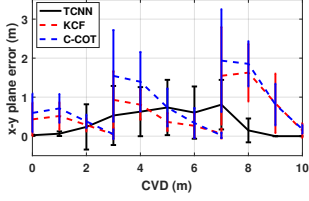
Figure 9: Tracking comparison with errors in meters.
