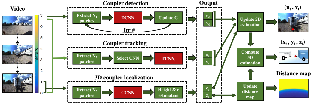
Figure 2: An automated computer vision system for coupler detection, tracking, and 3D localization.
