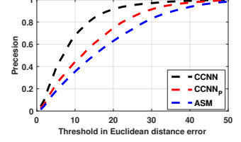
Figure 12: Contour estimation comparison.
