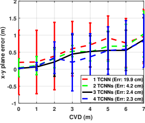
Figure 13: Number of TCNN networks used for tracking.
