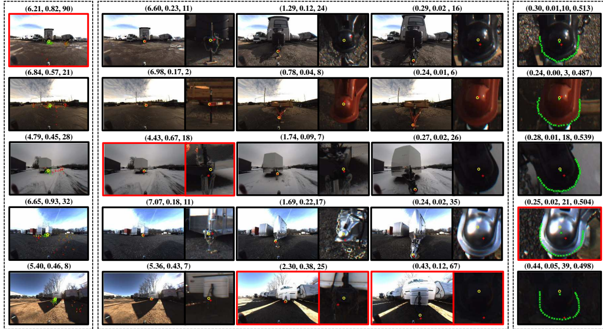
Figure 15: Qualitative results of five videos. The first column is the DCNN results, the three middle columns are TCNN results, last column is the CCNN result. Red + is the estimated result, yellow o is groundtruth, green x is the estimated contour. Above each frame is (CVD, meter error, pixel error), the last column also has the estimated height in meters. The red rectangles indicate the failure cases.
