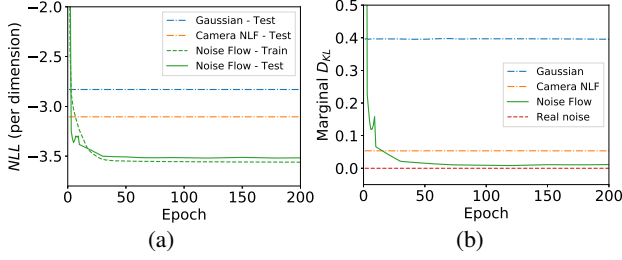
Figure 4: (a) NLL per dimension on the training and testing sets of Noise Flow compared to (1) the Gaussian model and (2) the signal-dependent model as represented by the camera-estimated NLFs. (b) Marginal KL divergence ( D_{KL} ) between the generated and the real noise samples.
