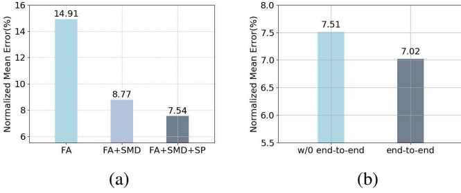
Figure 8: (a) Normalized Mean Error to analyze the effect of the pivotal components. (b) Normalized Mean Error to evaluate the effectiveness of alternate fine-tuning strategy.
