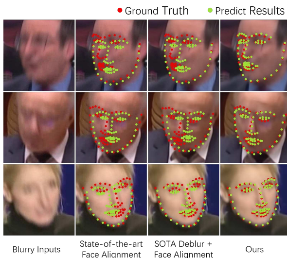
Figure 1: The first column is the frames of Blurred-300VW. In the second column, the results of state-of-the-art facial landmark detection algorithm are given. The third column corresponds to a naive combination of deblurring and facial landmark detection. In the fourth column are the results of our proposed algorithm.
