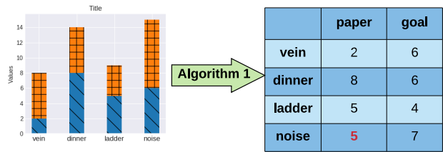
Figure 4. An example output of the chart to table algorithm. Red denotes incorrect predictions.
