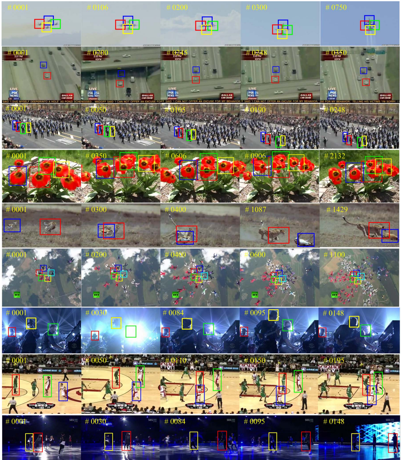
Figure 1. Tracking results obtained by mst-SPOT on all nine videos used in Experiment 1 (from top to bottom: Air Show , Car Chase , Parade , Red Flowers , Hunting , Sky Diving , Shaking , Basketball , and Skating ). The colors of the rectangles indicate the different objects that are tracked. Figure best viewed in color. Videos showing the full tracks are presented in the supplementary material.
