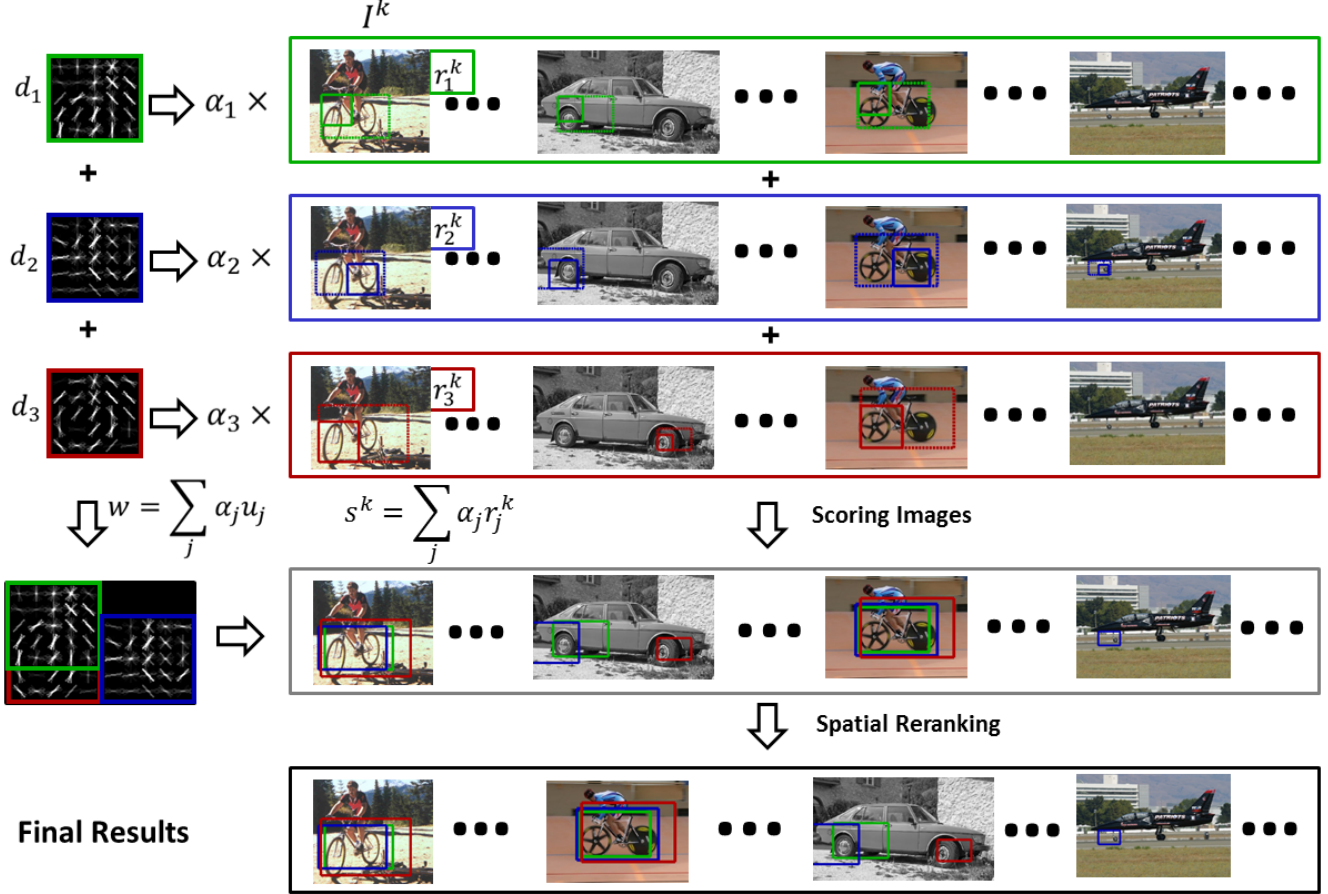
Figure 2. Detection using a template composed of CPs. Each CP retrieves a posting list of images, and a score for each image is computed from the weighted maximum response representation. Images are initially ranked on this score, and the top K then reranked using the spatial information associated with each maximum response.
