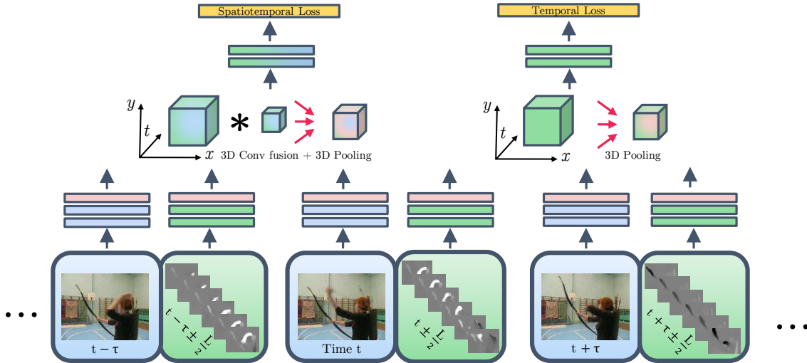
Figure 4. Our spatiotemporal fusion ConvNet applies two-stream ConvNets, that capture short-term information at a fine temporal scale ( t \pm \frac{\tau}{2} ), to temporally adjacent inputs at a coarse temporal scale ( t + T\tau ). The two streams are fused by a 3D filter that is able to learn correspondences between highly abstract features of the spatial stream (blue) and temporal stream (green), as well as local weighted combinations in x, y, t . The resulting features from the fusion stream and the temporal stream are 3D-pooled in space and time to learn spatiotemporal (top left) and purely temporal (top right) features for recognising the input video.
