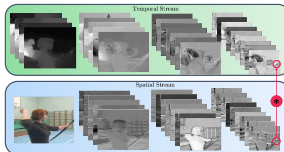
Figure 1. Example outputs of the first three convolutional layers from a two-stream ConvNet model [22]. The two networks separately capture spatial (appearance) and temporal information at a fine temporal scale. In this work we investigate several approaches to fuse the two networks over space and time.
