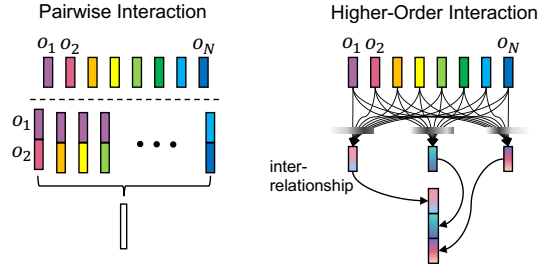
Figure 2. Typically, object interaction methods focus on pairwise interactions (left). We efficiently model the higher-order interactions between arbitrary subgroups of objects for video understanding, in which the inter-object relationships in one group are detected and objects with significant relationships (i.e. those that serve to improve action recognition or captioning in the end) are attentively selected (right). The higher-order interaction between groups of selected object relationships are then modeled after concatenation.
