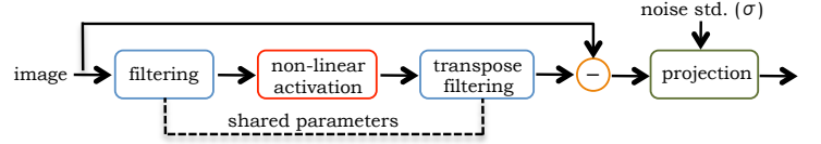
Figure 2. Schematic representation of the composite layer that serves as the core component of the proposed network architecture. Depending on the parametrization of the regularization operator, the filtering (transpose filtering) layer corresponds to either a convolutional or a non-local filtering layer.
