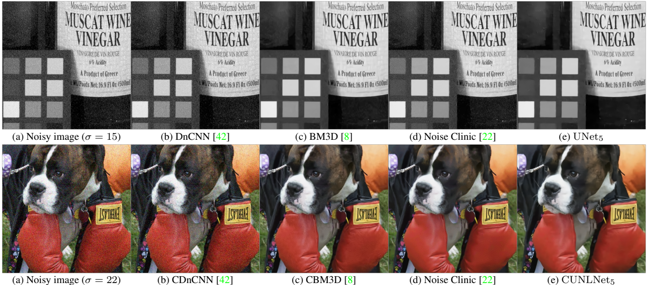
Figure 5. Real grayscale and color image denoising results. The indicated value of \sigma corresponds to noise’s standard deviation estimate, which we provide as additional input both to BM3D and to our proposed networks. The details in the results are better viewed magnified on a computer screen.
