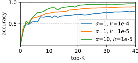
Figure 7. Performance of our weighted soft-margin triplet loss with different parameters. lr is short for learning rate. It takes about 1 hour to train each epoch.
