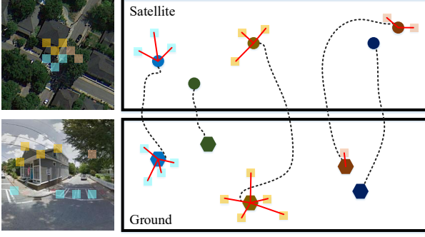
Figure 3. An illustration of how NetVLAD achieves cross-view matching. (Top): satellite view, (Bottom): ground view. In each view, there are a set of local features (colorful squares) and their associated centroids (hexagons and circles). After training, each centroid of satellite view is associated with the unique centroid of ground view (dotted lines). The residuals (red lines) are independent to their own views and comparable to the other view because they are only relative to the centroids. Thus, the global descriptors, i.e. aggregated residuals, of two views are in the common space.
