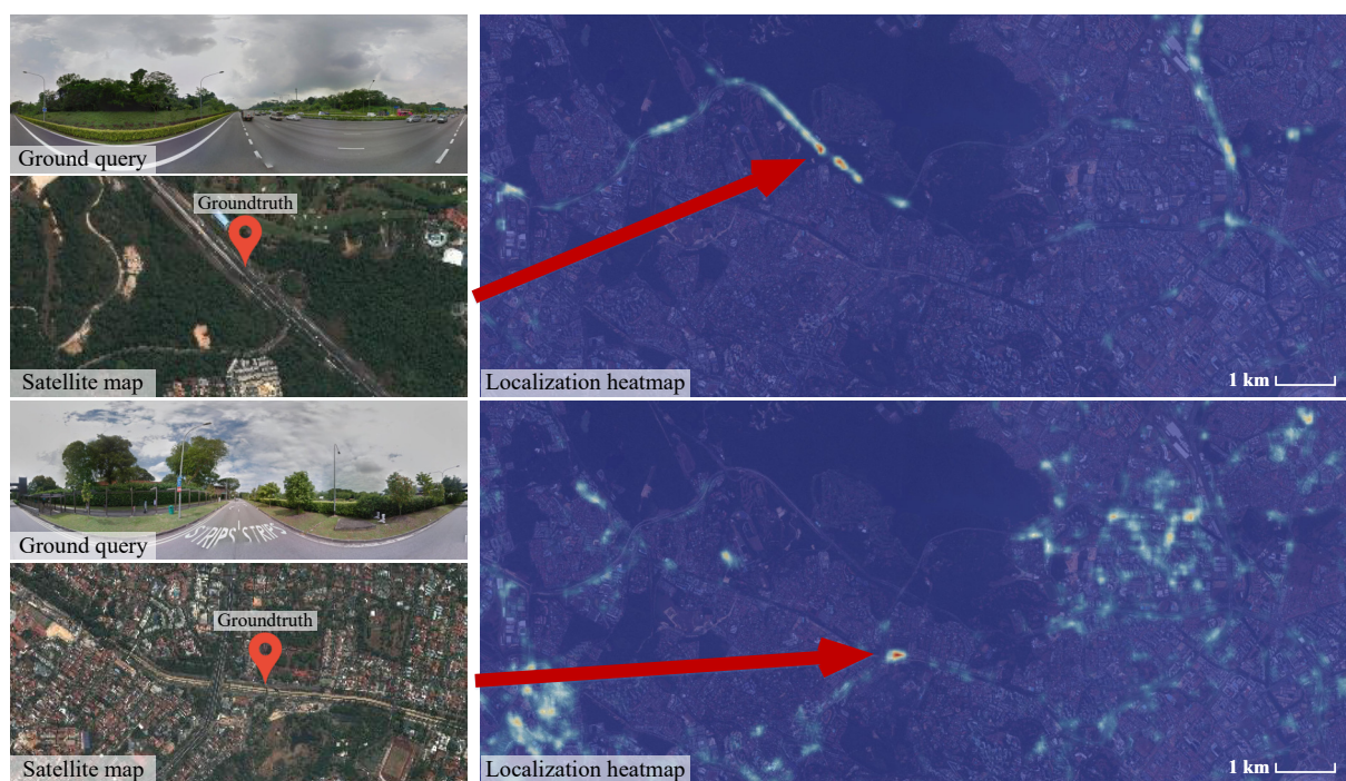
Figure 10. Large-scale geo-localization examples on our dataset.
