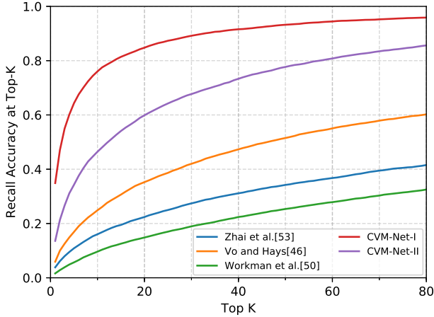
Figure 5. Comparison of our CVM-Nets and other existing approaches [53, 46, 50]: All models are trained on CVUSA [53].
