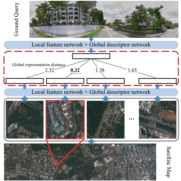
Figure 1. An illustration of the image based ground-to-aerial geo-localization problem, and our proposed framework.
