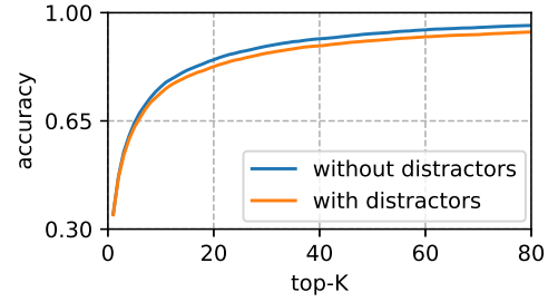
Figure 6. Top-K recall accuracy on the evaluation dataset with and without distractor images. The model is trained on CVM-Net-I on CVUSA dataset [53].
