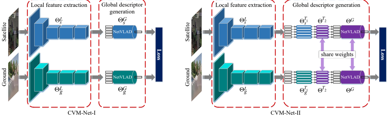
Figure 2. Overview of our proposed CVM-Nets. CVM-Net-I : The deep network with two aligned (no weight-shared) NetVLADs which are used to pool the local features from different views into a common space. CVM-Net-II : The deep network with two weight-shared NetVLADs that transform the local features into a common space before aggregating to obtain the global descriptors.
