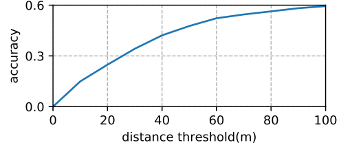
Figure 8. The retrieval accuracy on distance error threshold.
