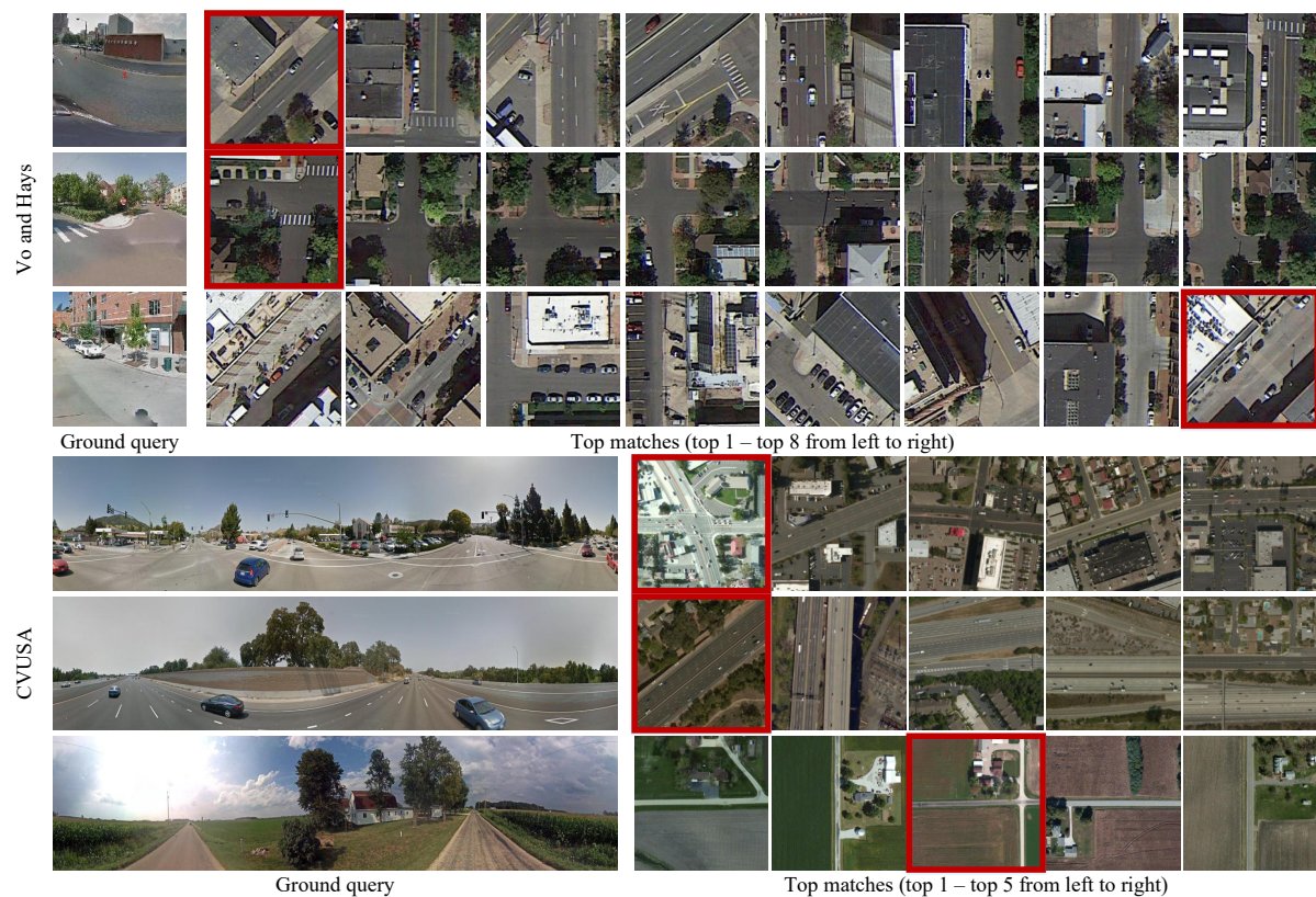
Figure 9. Image retrieval examples on Vo and Hays dataset [46] and CVUSA dataset [53]. The satellite image bordered by red square is the groundtruth.
