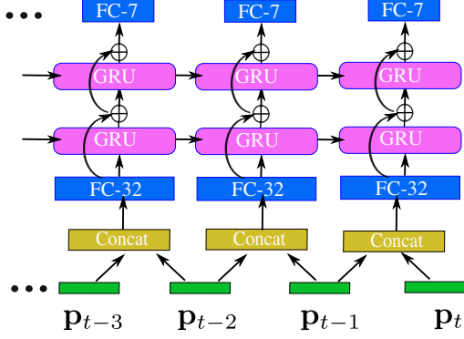
Figure 3: The GRU RNN network architecture for modeling a sequence of camera poses.
