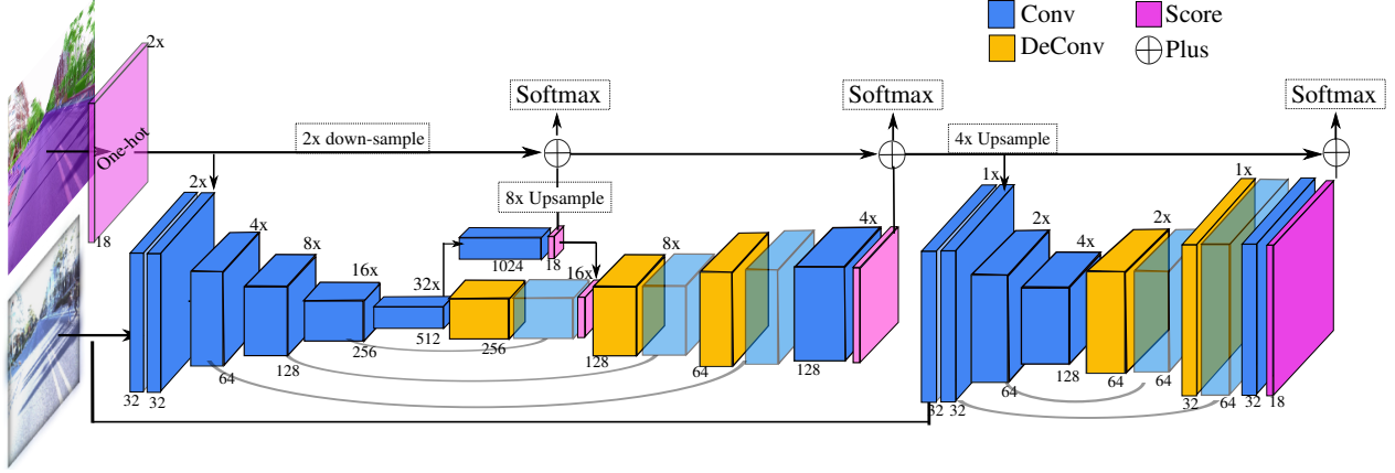
Figure 4: Architecture of the segment CNN with rendered label map as a segmentation priori. At bottom of each convolutional block, we show the filter size, and at top we mark the downsample rates of each block w.r.t. the input image size. The ‘softmax’ text box indicates the places a loss is calculated. Details are in Sec. 4.3.
