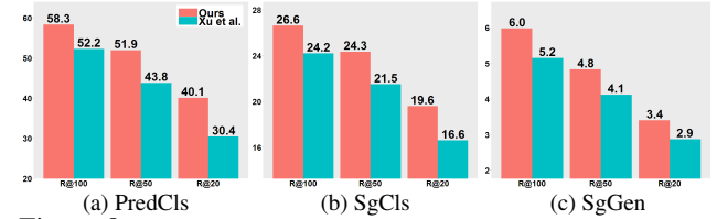
Figure 8: Scene graph detection task (see Table 1) results on Visual Genome using ours (red) and [52] (cyan). Our pipeline without the RL module show results similar to [52] (cyan).
