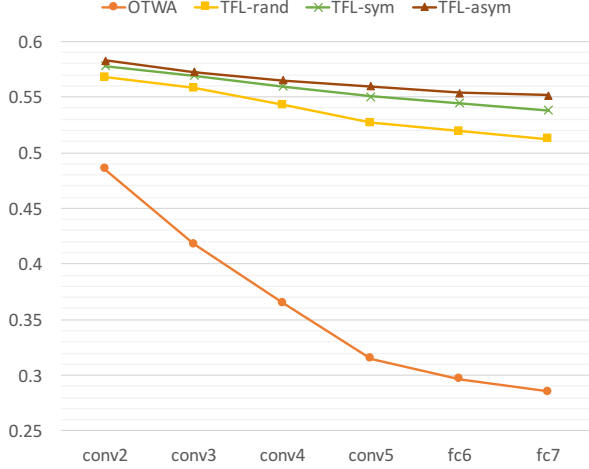
Figure 1. Top-1 accuracy after each layer is quantized for different transformation function learning settings. The results are conducted based on the SQ-2 AlexNet mode without fine-tuning.
