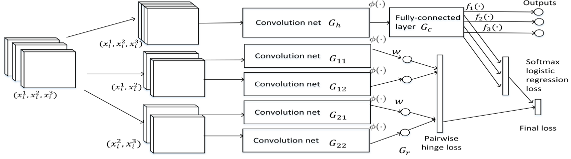
Figure 1: The architecture of CNNPOR for a 3-rank ordinal regression problem.
