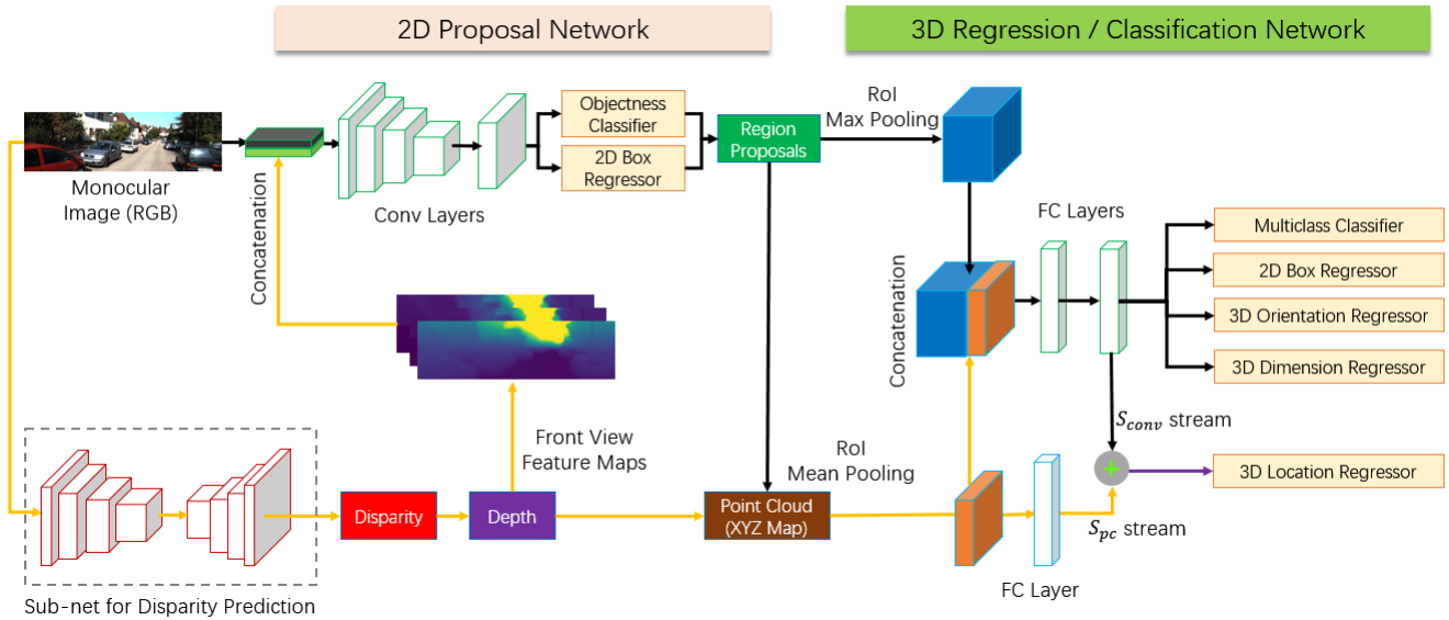
Figure 1. The proposed framework for 3D object detection.
