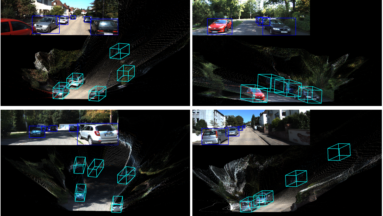
Figure 3. Visualization for 2D detection boxes, the projected 3D detection boxes on inferred point cloud from estimated disparity.
