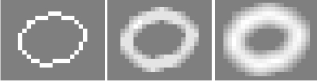
Figure 2: Example of “submanifold” dilation. Left: Original curve. Middle: Result of applying a regular 3 \times 3 convolution with weights 1/9 . Right: Result of applying the same convolution again. Regular convolutions substantially reduce the feature sparsity with each convolutional layer.
