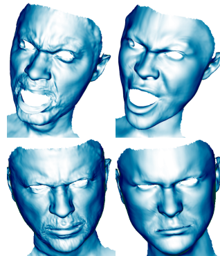
Figure 6. Visual results for shape-from-shading for images from [31]. From left-to-right: rendered mesh ( LINEAR ), rendered mesh (OURS). Note: for original images, please refer to [31].
