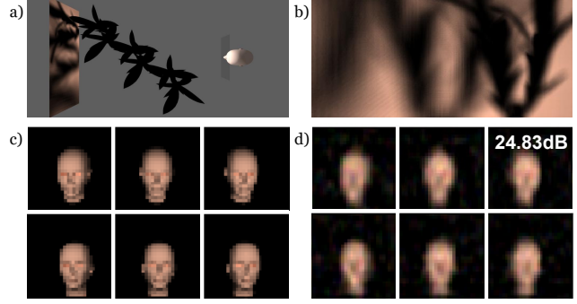
Figure 7: Recovered light field of another simulated scene, using the same occluder as in scenario (f) of Fig. 5. (a) Simulated scenario and (b) the resulting observation. In (c) we show selected views from the ground truth light field and in (d) the same views for the recovered light field. This illustrates the performance of our method for an arbitrary scene, with self-occlusions and non-planar elements.
