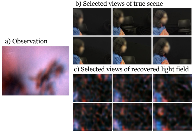
Figure 10: Reconstructions of an experimental scene with a seated subject at the scene plane. (a) Observation plane after background subtraction. (b) Six views of the true scene, captured in the same manner as in Fig. 9 (c) Reconstructions of the light field for the same views as in (b).
