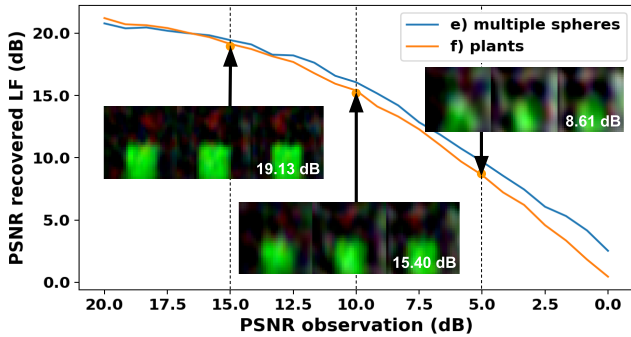
Figure 6: Reconstruction PSNR plotted against observation PSNR, for simulated scenarios (e) and (f) from Fig. 5. We also show three reconstructions of the scene using the setup from (f), for three different values of the PSNR.
