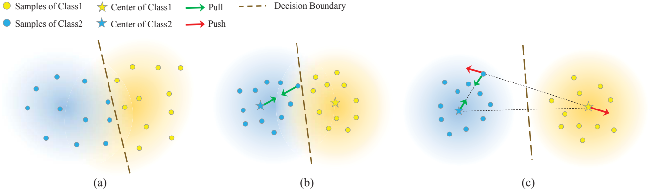
Figure 2. A toy illustration of the distributions of deep features learned by (a) softmax loss, (b) center loss + softmax loss, and (c) triplet-center loss + softmax loss. Intuitively, the decision boundary of the softmax classifier separates the two classes elaborately. The center loss pulls features toward their corresponding centers. The TCL pulls the features to their corresponding centers and pushes the features away from the other centers.
