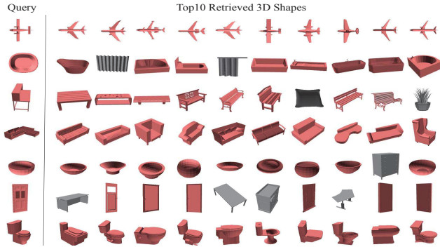
Figure 5. Retrieval examples on ModelNet40 dataset. Top matches are shown for each query with mistakes highlighted in gray.
